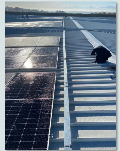
30kWp DC Grid Tie Install
